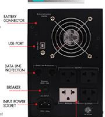
OUTPUT SOCKET
