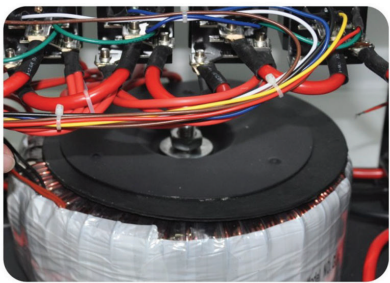
Toroidal Transformer
