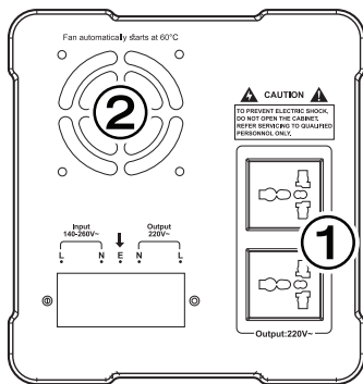
HDR-3000VA HDR-5000VA
